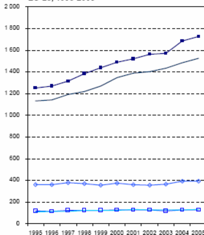
Fig. 4: Evolution of freight transport (in billion tonne-kilometres performed*), by transport mode**, EU-25, 1995-2005
